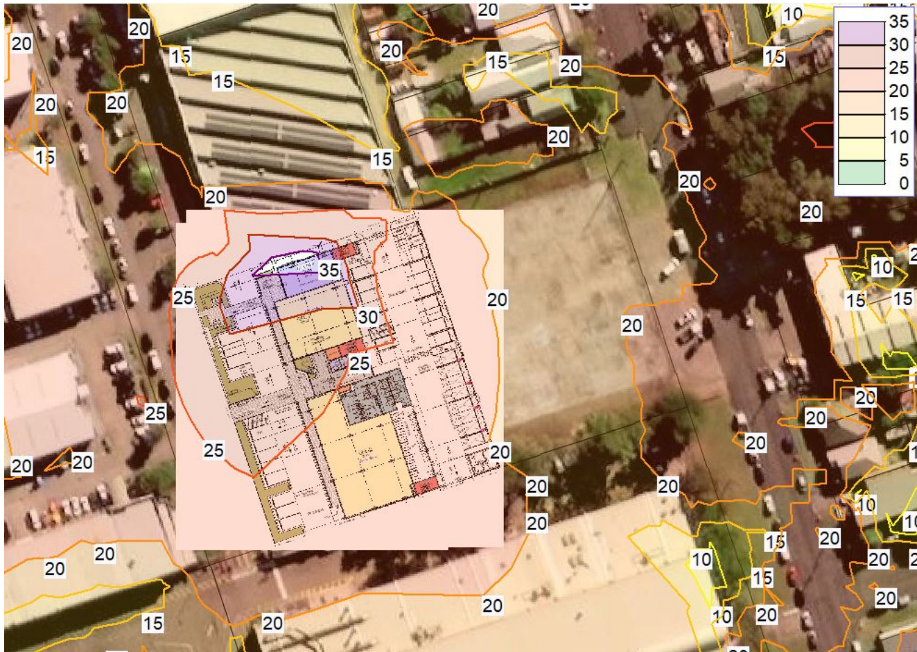
Figure 10 Cumulative Operational Noise Modelling Results dB(A) Leq(15min)
